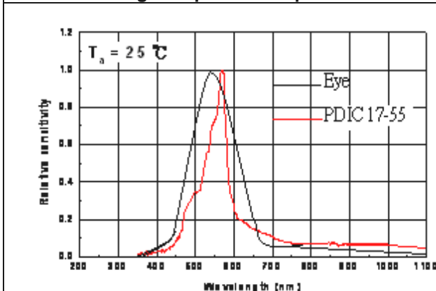
Fig.9 Spectral Response
