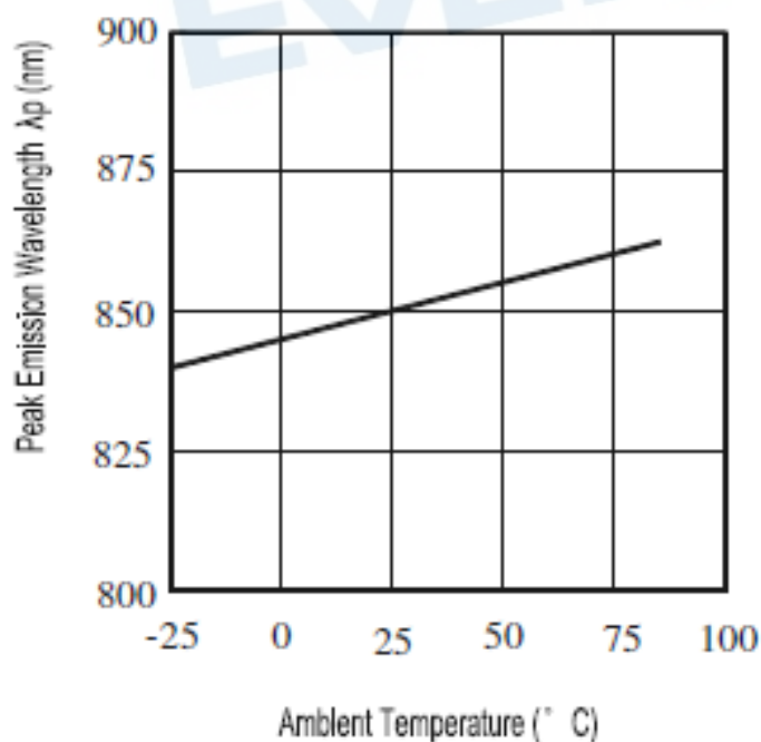
Fig.3 Peak Emission Wavelength Ambient Temperature
