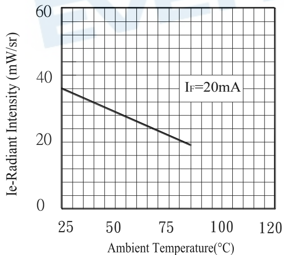
Fig.7 Radiant Intensity vs. Ambient Temperature(°C)
