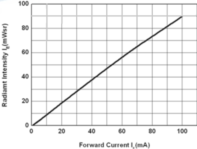
Fig.4 Relative Intensity vs. Forward Current
