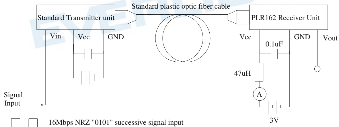
*Fig.2 Measuring Method of Dissipation Current
