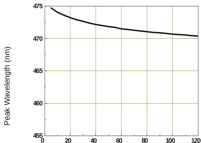
Dominant Wavelength vs. Forward Current ( T_a=25^\circ\text{C} )
