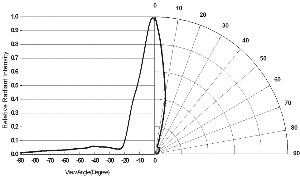
Relative Radiant Intensity vs. Angular Displacement
